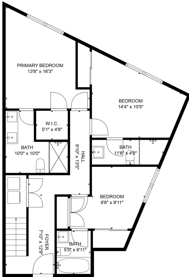
FLOOR 1
