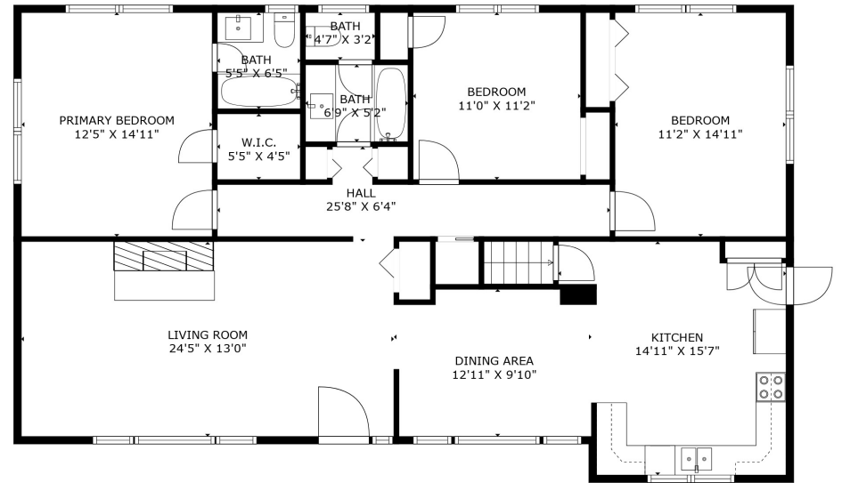
FLOOR 2
