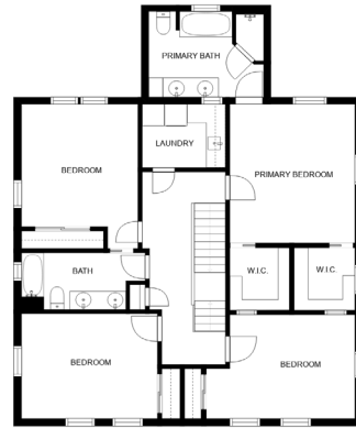
FLOOR 3
