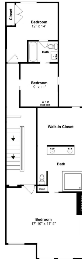
Third Floor
