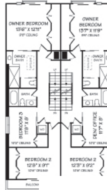
UNIT 3 SECOND LEVEL 10'6" VAULTED CEILING
